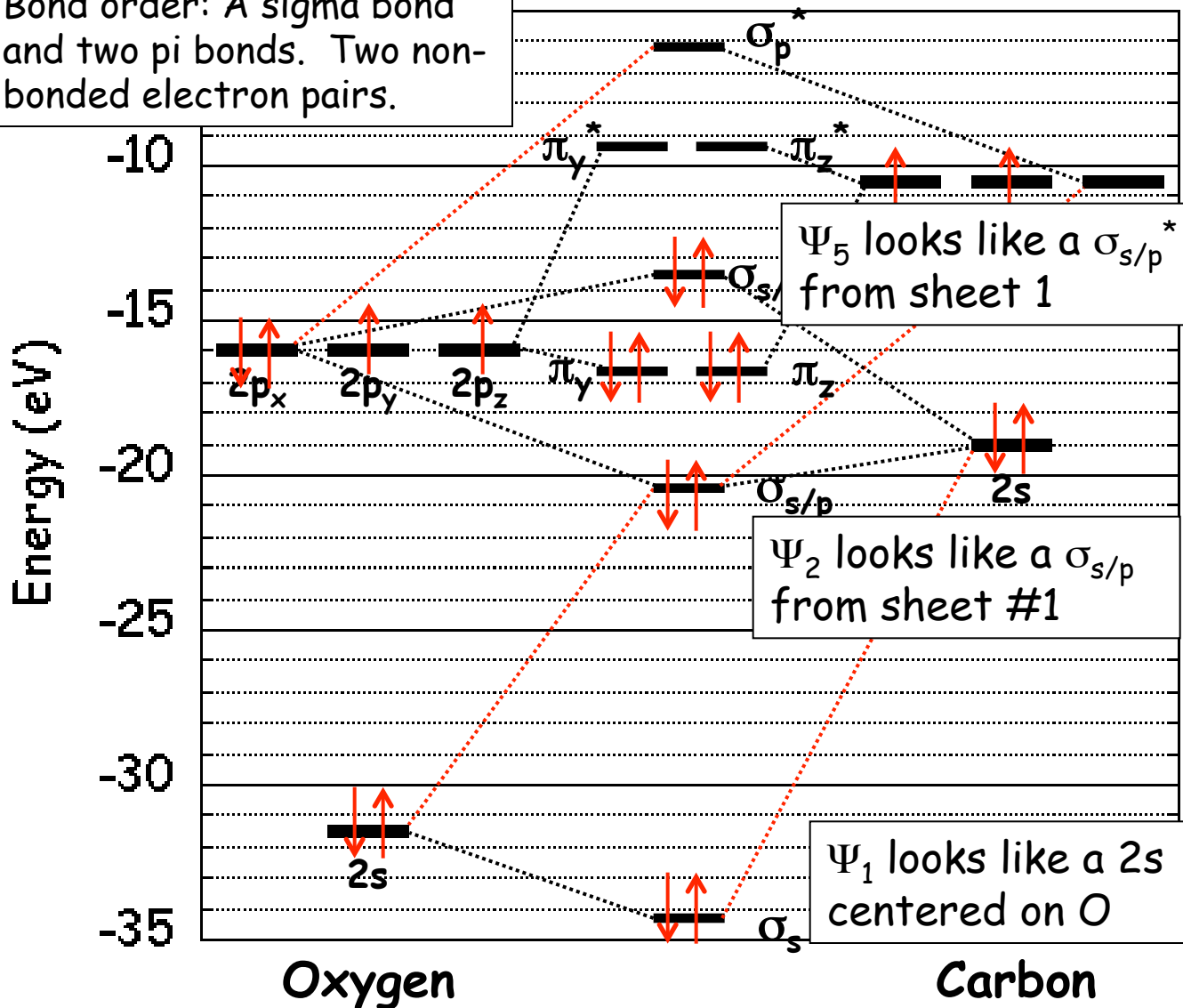
Carbon Monoxide Orbital Interaction Diagram
